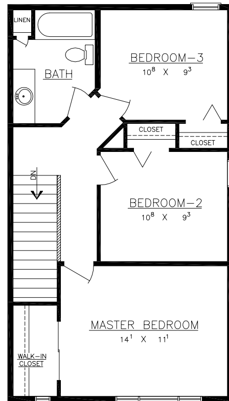
SECOND FLOOR PLAN AREA = 597 S.F.
